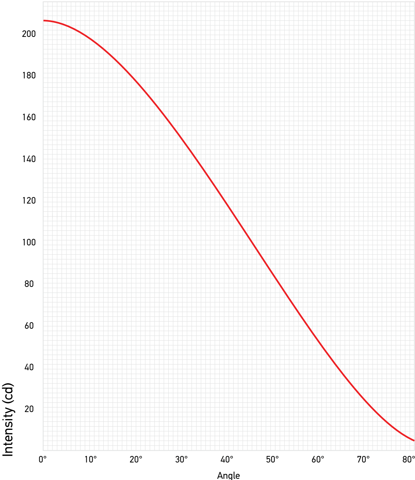
EuroLED 95 White Light Candela Output
